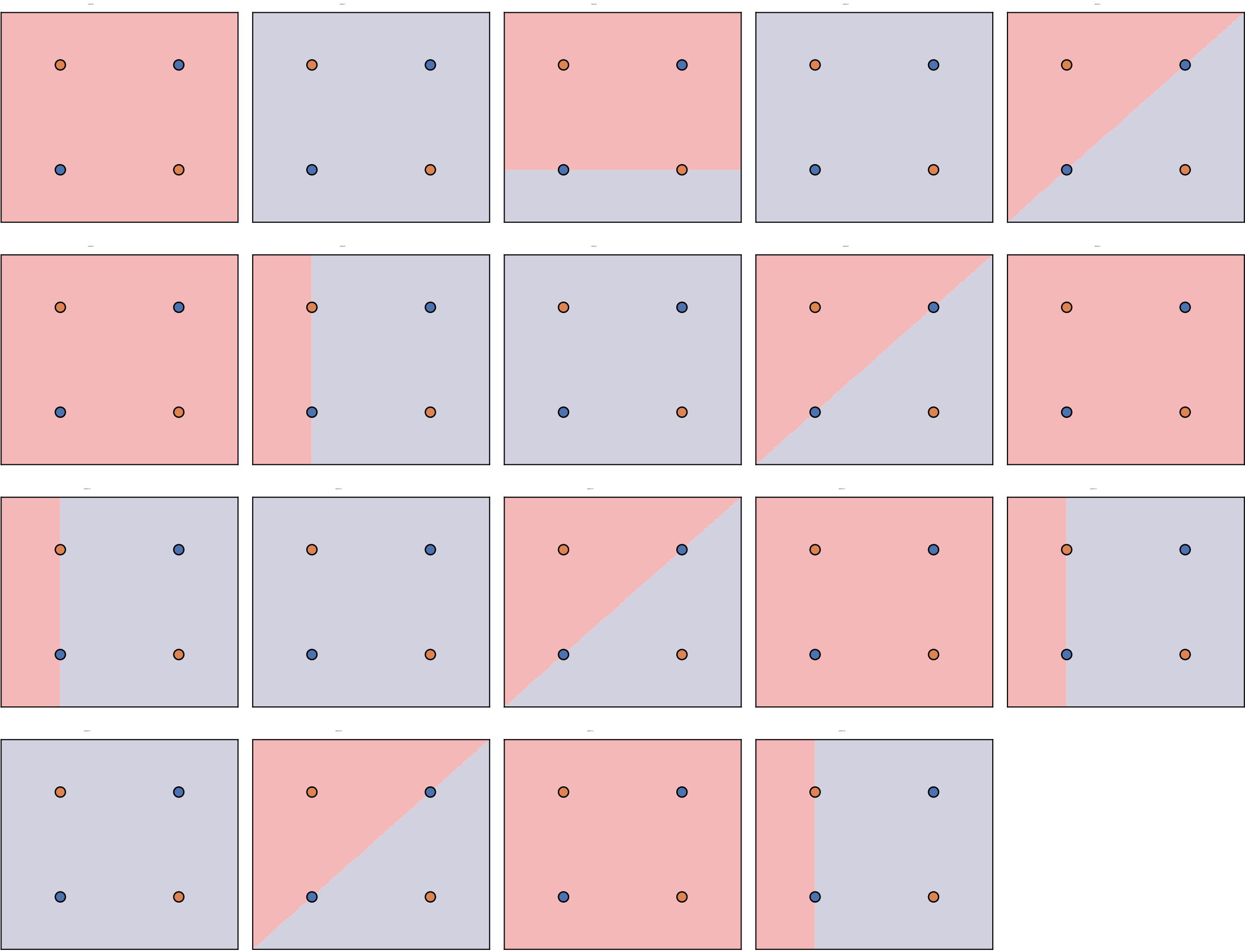
80% Decision Boundary After Each Weight Update
